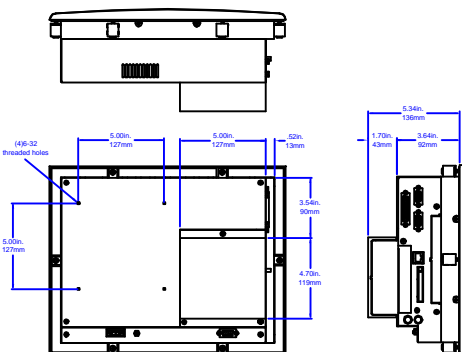
P1 10" with COV-3000-A
