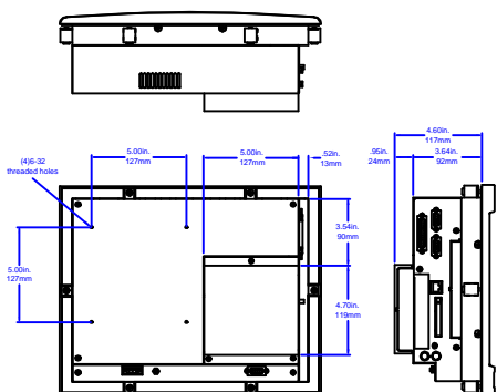
P1 10" with COV-2000-A
