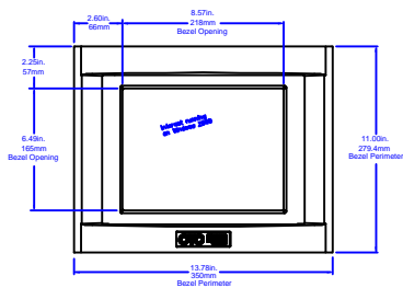
P1 10" Front View
