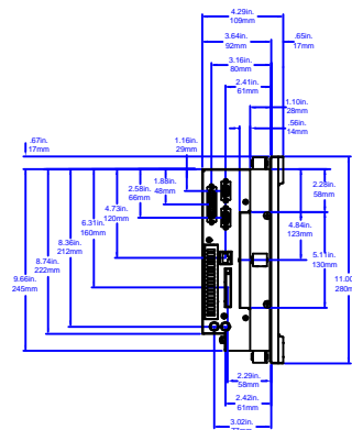
P1 10" Left Side View
