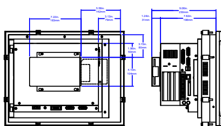
PS15-3/4 with FLP-2000-A
