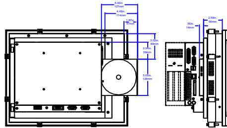
PS15 CD ROM Drawer Extension
