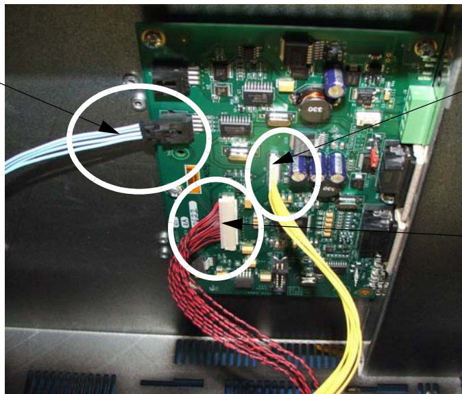
Figure 8: Accessing the 17" Monitor Cables
