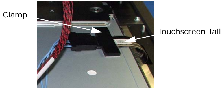
Figure 9: Lift the Clamp to Disconnect the Touchscreen Tail
