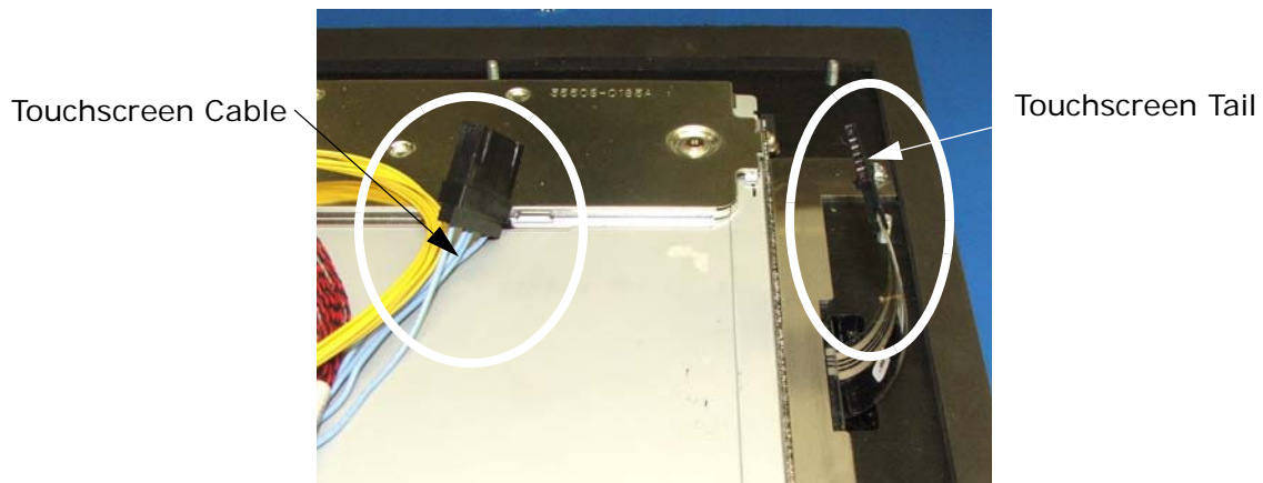
Figure 10: Disconnecting the Touchscreen Cable
