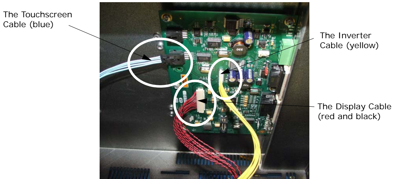
Figure 3: Accessing the 15" Monitor Cables
